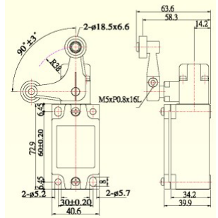
MJ-3244 Metal limit switch, 2 screws, IP67 MJ-3244-M Metal limit switch, 3 screws, metal roller, IP67
