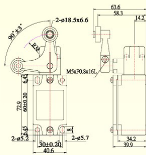
MJ-3242 Metal limit switch, 2 screws, IP67 MJ-3242-M Metal limit switch, 3 screws, metal roller, IP67
