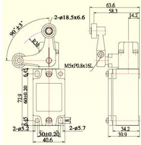
MJ-3241 Metal limit switch, 2 screws, IP67 MJ-3241O Metal limit switch, 3 screws, IP67 MJ-3241-M Metal limit switch, 2 screws, metal roller, IP67
