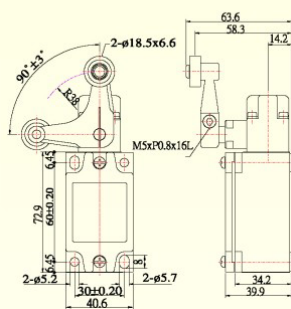
MJ-3243 Metal limit switch, 2 screws, IP67 MJ-3243-M Metal limit switch, 3 screws, metal roller, IP67
