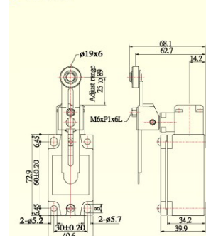
MJ-7108 Metal limit switch, 2 screws, IP67 MJ-7108O Metal limit switch, 3 screws, IP67 MJ-7108-P Metal limit switch, plastic roller, IP67 MJ-7108-26 Metal limit switch, 50 mm big rubber roller
